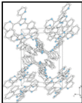
Fig. 2. A view of the crystal packing of the title compound, viewed along the a axis. Hydrogen atoms have been omitted for clarity.
