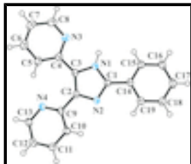
Fig. 1. A view of the molecular structure of the title compound, showing 50% probability displacement ellipsoids for the non-hydrogen atoms.
